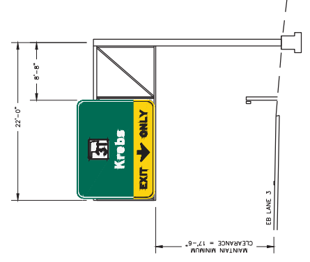
OHS4 EXISTING OHS STRUCTURE @ 22' US-270/SH-1/SH-31 EASTBOUND
